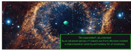
The Helix Nebula, NGC-7293, as seen through the Hubble Telescope. Located 650 light years from Earth, in the constellation Aquarius. Also known as The Eye of God.
